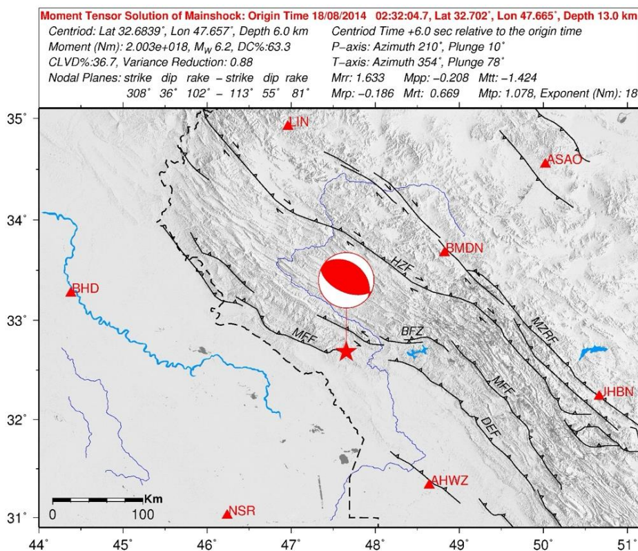
Figure 4. The outcomes for the favored MT solution in the main-shock M_w 6.2. The details of the moment tensor solution, nodal planes and etc. are presented in the box above the figure. The red triangles show the seismic stations used in MT inversion.
