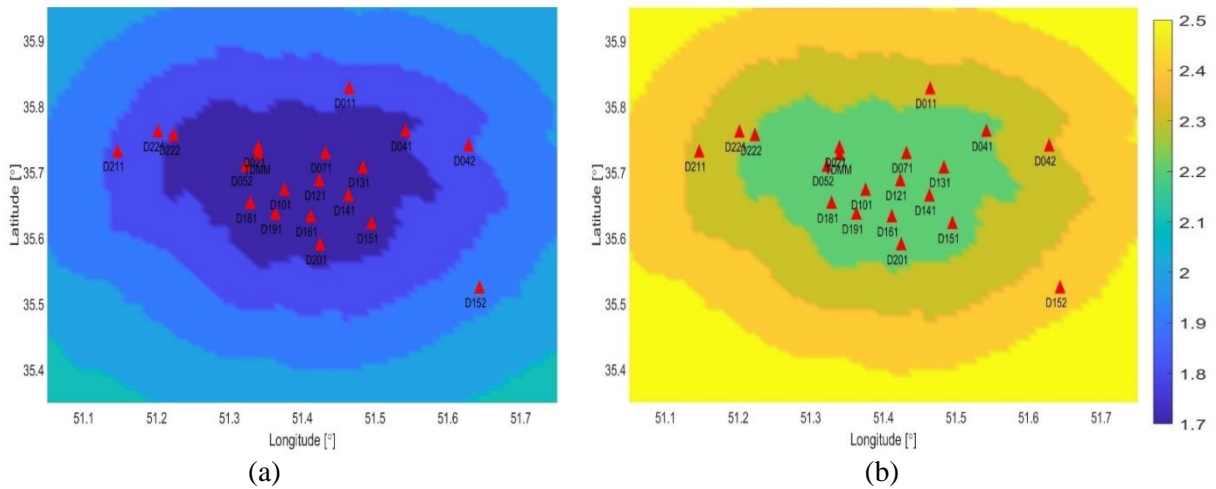
Figure 4. The detection threshold map with a constant noise level, station D071 as reference, at a depth of 10 km for (a) S-wave, and (b) P-wave.
