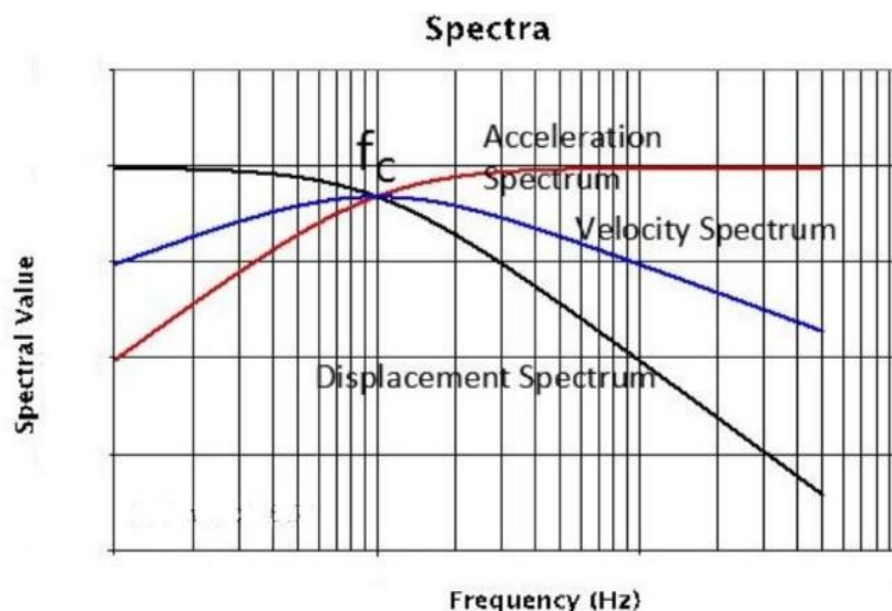
Figure 1. The schematic Fourier Amplitude Spectrum of strong earthquake acceleration (Ding, 2015).
