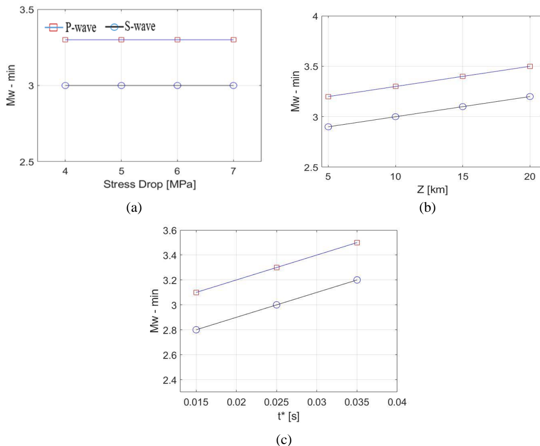
Figure 5. Variability of the detection threshold for P- and S-waves as a function of (a) the stress drop, (b) the focal depth, and (c) the reduced time ( t^* ). Changes in the stress drop do not affect the magnitude of the threshold (a), while changes in focal depth from 5 to 20 km cause changes as large as 0.3 units in magnitude of the threshold (b), and changes in t^* from 0.015 to 0.035 sec cause changes as large as 0.4 units in the magnitude of the threshold (c).
