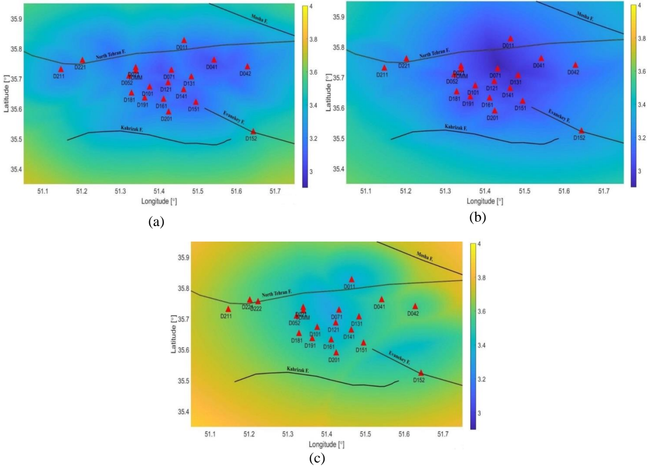
Figure 3. The detection threshold map at a depth of 10 km for the (a) E-component of the S-wave (b) N-component of the S-wave, and (c) Z-component of the P-wave.
